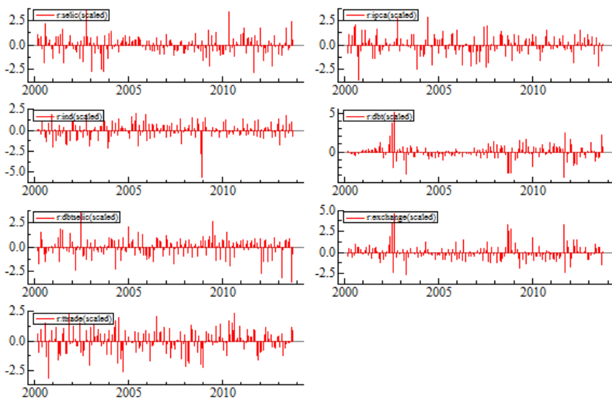
Figure 2 - MS-VAR residuals
