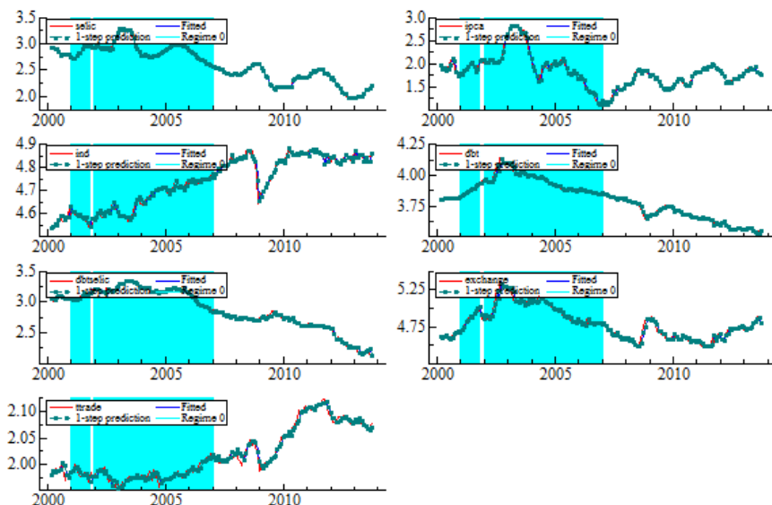
Figure 4 - Model fit for regimes
