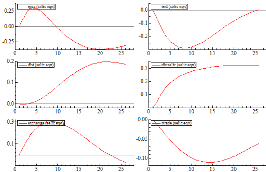
Figure 7 - Impulse-response function dependent on Regime 2 (shock of one percentage point in the Selic)
