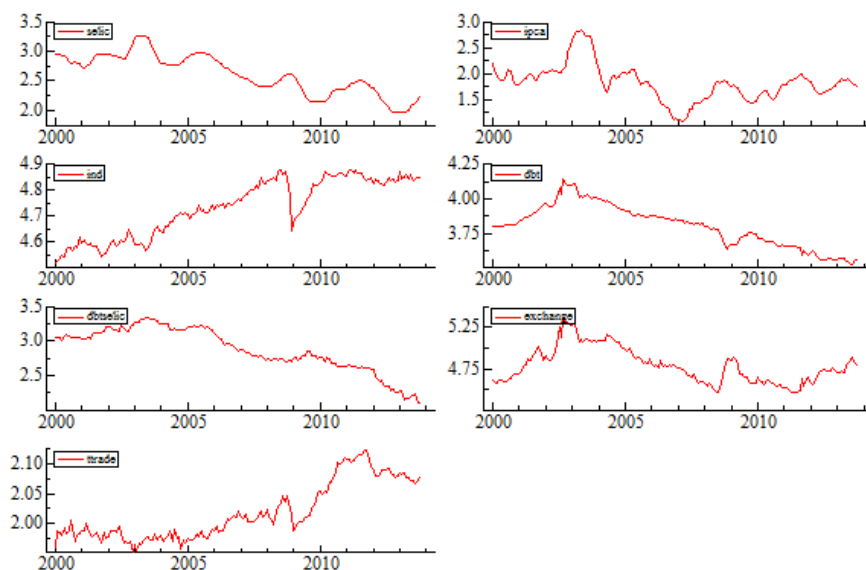
Figure 1 - Behavior of the selected variables over time
