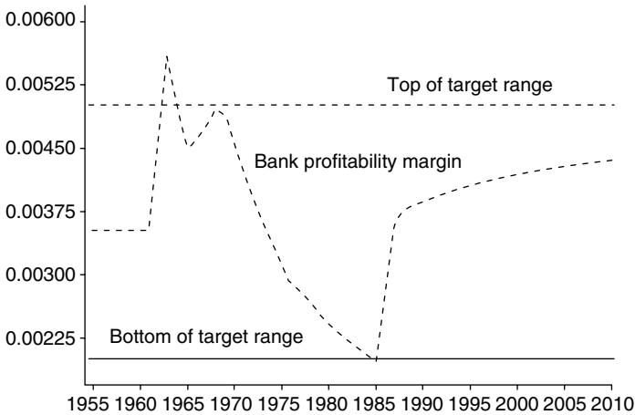
Figure 10.2I Evolution of the bank profitability margin, relative to its target range, following a one-step permanent increase in real government expenditures
