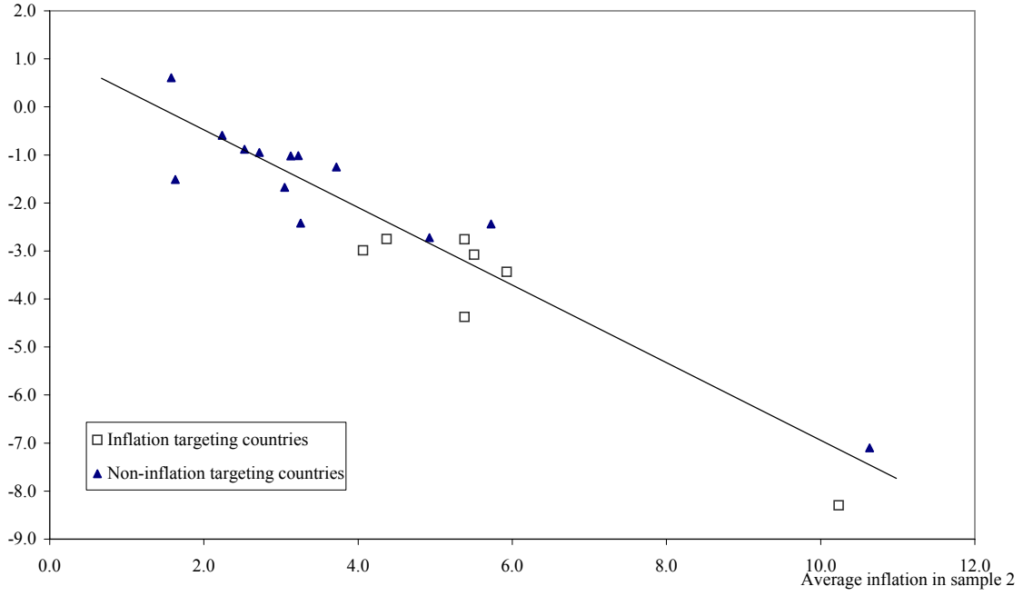
Figure 1: Regression to the mean
